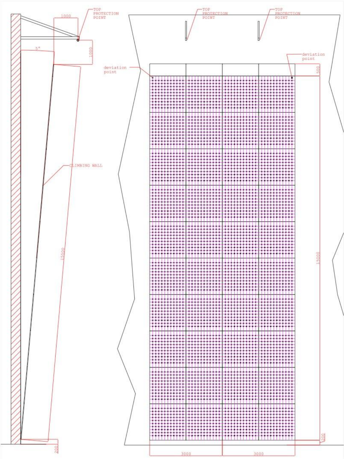
Figure 8.2(b) (Climbing lane design for the 15m Event)
