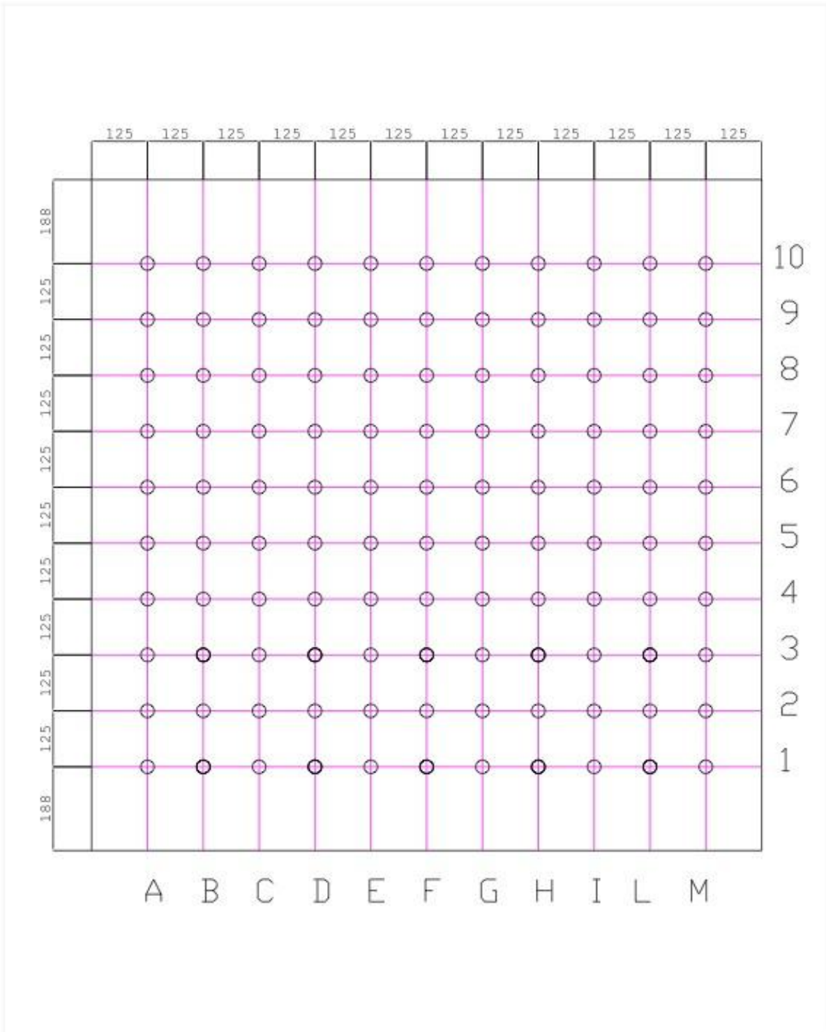
Figure 8.2(c) (M10 insert grid for each panel on the climbing surface)
